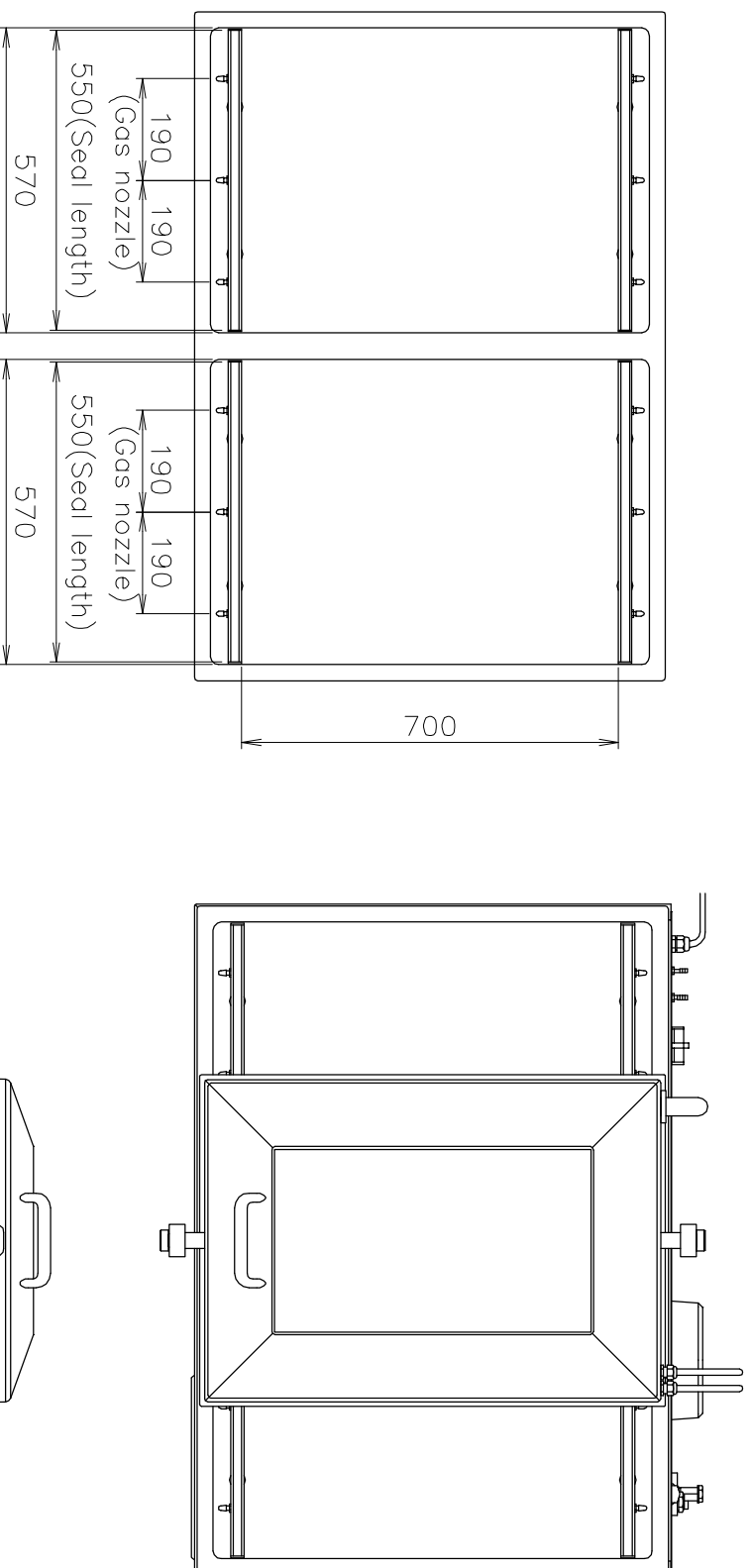
Chamber detail
