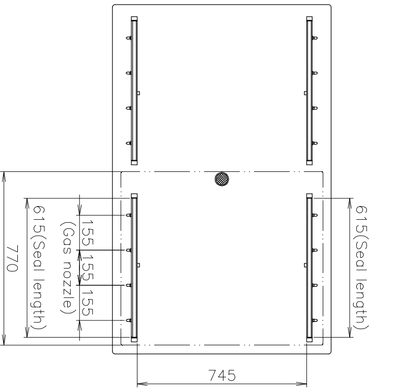
Chamber detail
